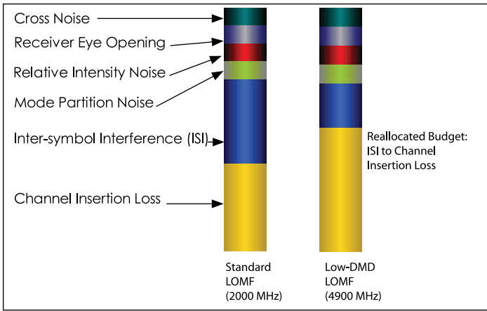
Figure 4. 75% of the total loss budget is allocated to ISI and channel insertion loss in IEEE 802.3ae.
