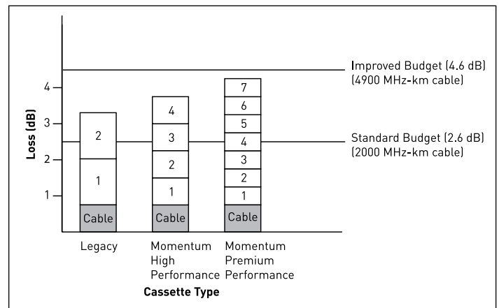
Figure 5. Low DMD cable and improved cassettes can allow more connections in the channel.
