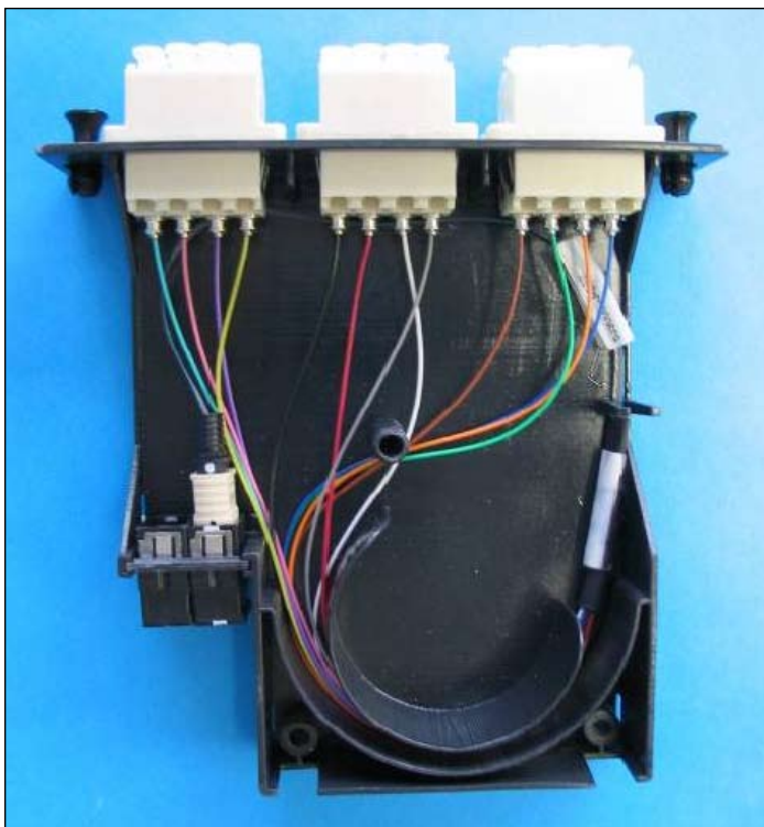
Figure 2. A fiber cassette acts as a transition between a MTP/ MPO-based multi-fiber backbone and LC- or SC-terminated patch cords (shown with cover removed for clarity).
