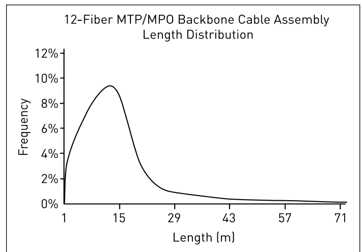
Figure 6. Most backbone cables in a DC are much shorter than the 300 meters maximum allowed by standards and the 600 meters possible with such cables as the GIGALite-XB.
