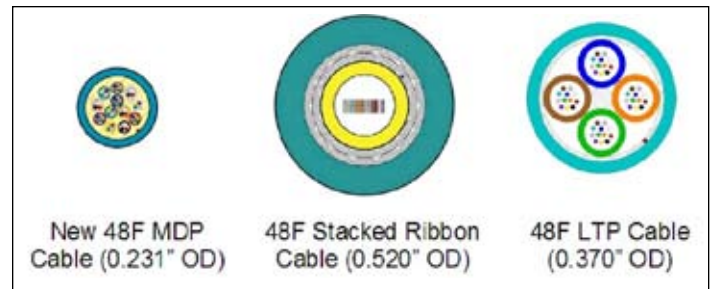
Figure 1. Reduced-diameter cables save space in crowded conduits.
