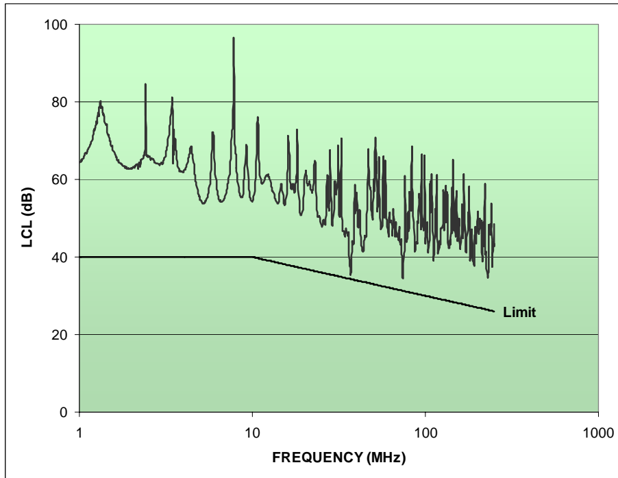
Figure 2: LCL measurement for worst category 6 cable
