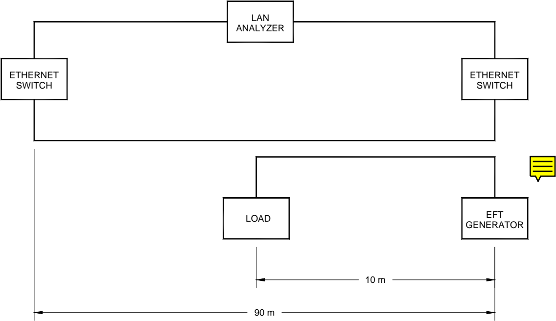
Figure 1: EFT noise immunity test setup
