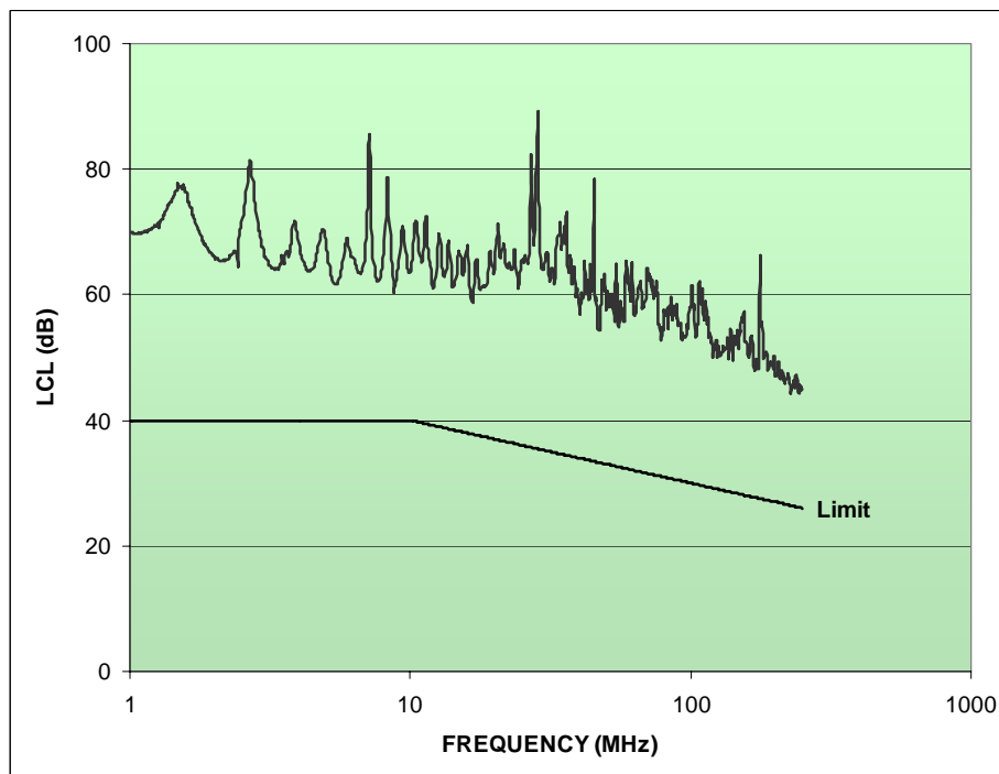
Figure 3: LCL measurement for best category 6 cable
