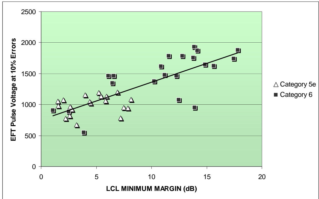
Figure 5: Correlation of EFT noise immunity and LCL measurements
