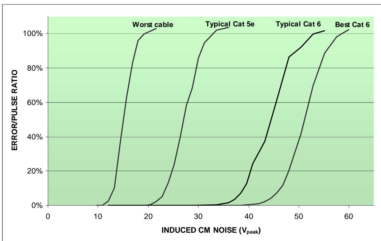
Figure 4: EFT noise susceptibility measurements
