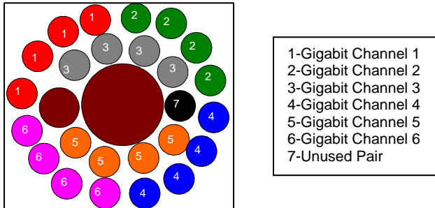
Figure 1: 6 Gigabit Ethernet Configuration
